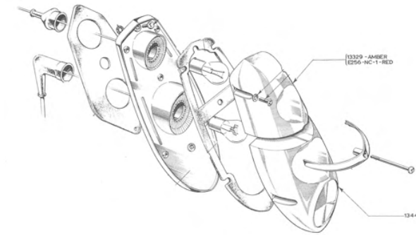
REAR LAMP AND REAR FLASHER-ESTATE CAR
