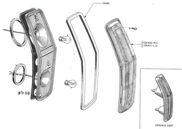
REAR LAMP and FLASHER STATION WAGON
